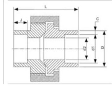
Socket Union
