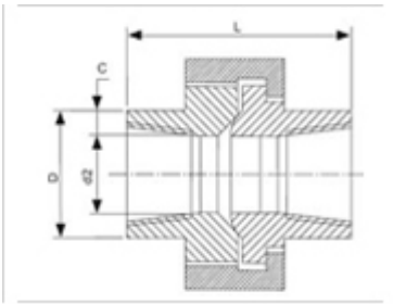
Threaded Union
