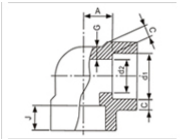
90° Elbow
