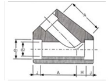
Lateral
