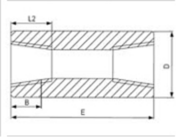
Coupling
