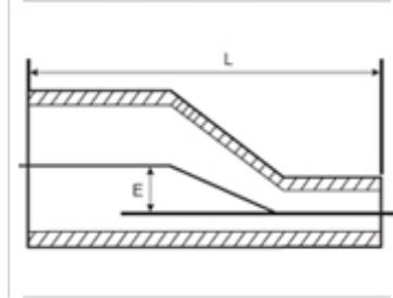
Eccentric Swaged Nipple
