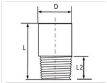
Round Head Plug
