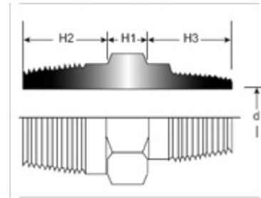
Reducing Hex Nipple
