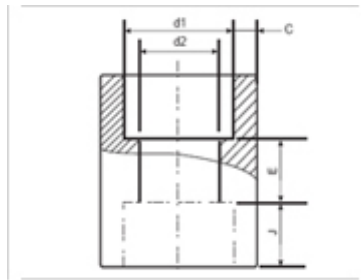
Half Coupling
