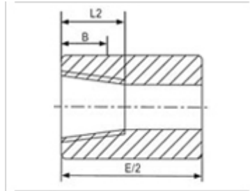
Half Coupling
