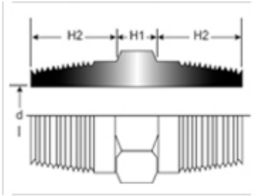
Hex Nipple
