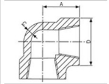
90° Elbow
