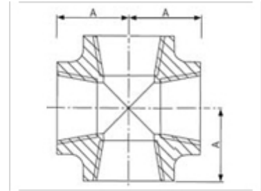
Cross
